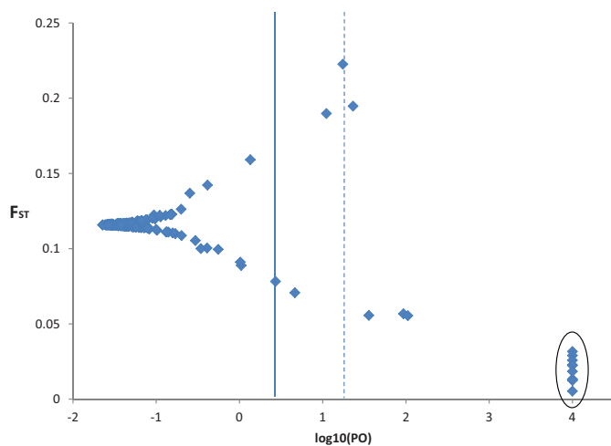
FIGURE 3. Results of F_{ST} outlier test based on differentiation in nonnative Brook Trout in Idaho and putative hatchery source populations as implemented in BayeScan. Eighteen markers fell above the targeted false discovery rate (FDR) of 0.01 (vertical dashed line) and were considered “outliers,” and 10 markers (circled) fell at the extreme end of this distribution. One hundred and thirty-seven loci fell below the FDR of 0.05 (solid vertical line) and were retained for a “neutral” data set. [Figure available online in color.]
