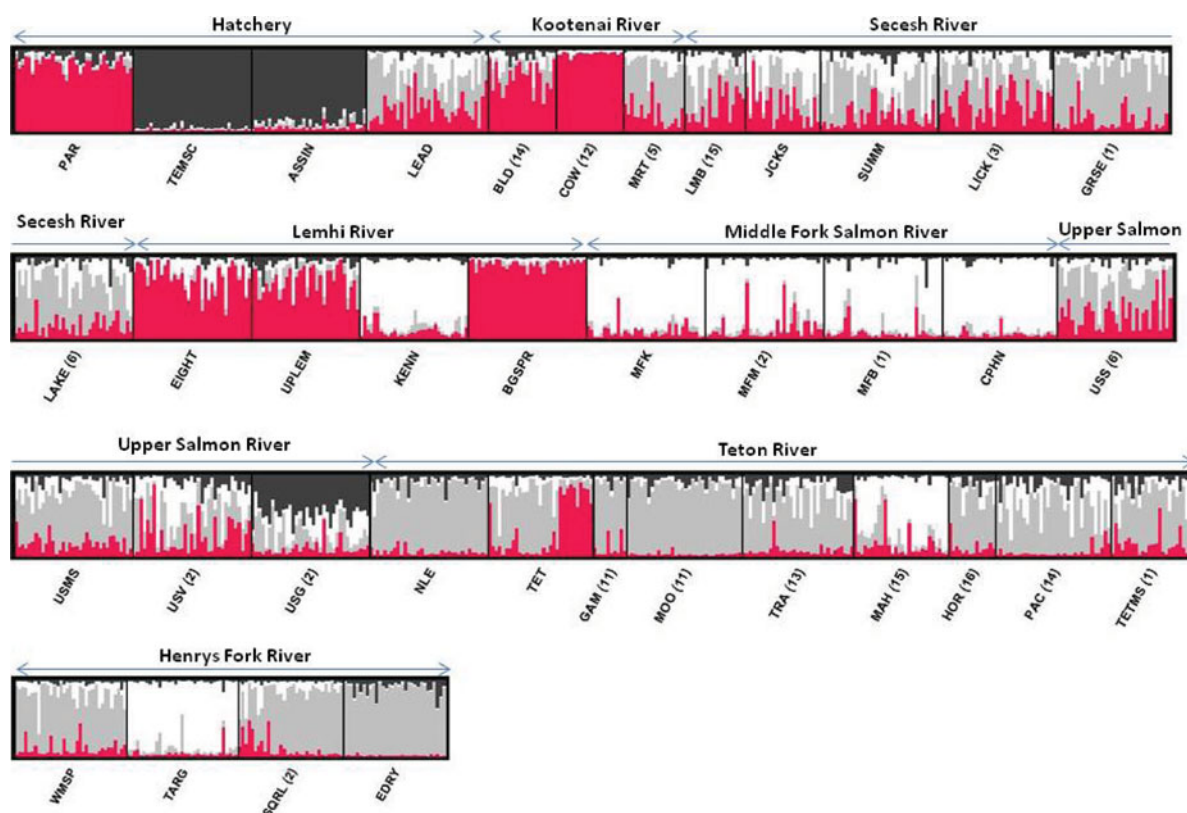
FIGURE 5. STRUCTURE results based on four clusters ( k = 4 ) for samples from four hatcheries and from populations of nonnative Brook Trout across Idaho. Ten runs were implemented using 500,000 burn-in iterations and 500,000 MCMC repetitions. Individual assignments were aligned using the program CLUMPP (see text). Colors (red, light grey, dark grey, and white) represent the four clusters defined by STRUCTURE, and each vertical bar shows the proportional ancestry ( Q ) within an individual fish in each cluster. Dark vertical lines separate samples, names of which are abbreviated below each sample (see Table 1 for definition of abbreviations); origin (i.e., hatchery or major watershed) is given above. Where stocking was historically recorded, the number of stocking events is shown in parentheses. [Figure available online in color.]
