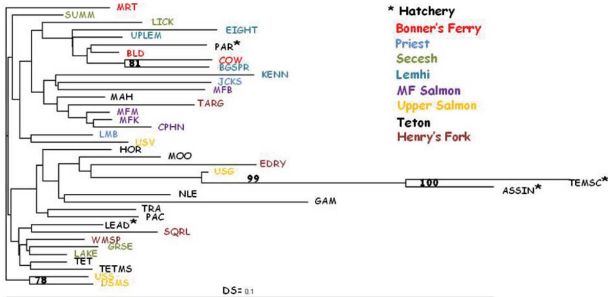
FIGURE 4. Neighbor-joining phenogram using Nei's genetic distance ( D ). Population abbreviations are defined in Table 1 and are colored by major drainage or hatchery origin described at the right of the figure. Bootstrap values > 50 (percent out of 500 iterations) are shown. [Figure available online in color.]
